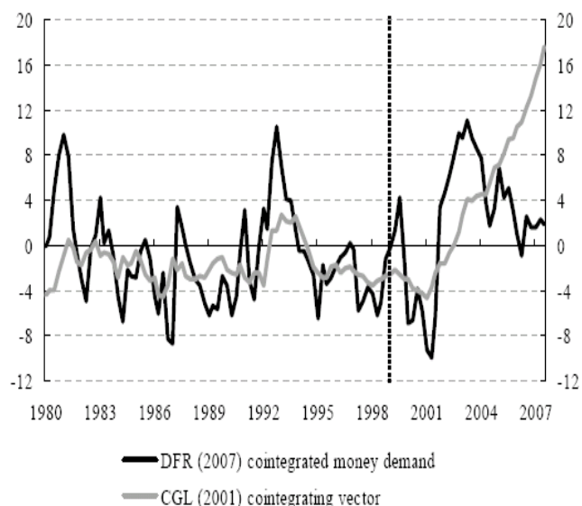
Figure 2: Residual of a standard money demand specification based on Calza et al. (2001) and de Santis et al. (2013).
